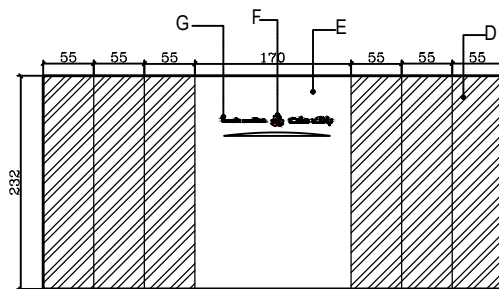
VIEW-C SC 1:20
