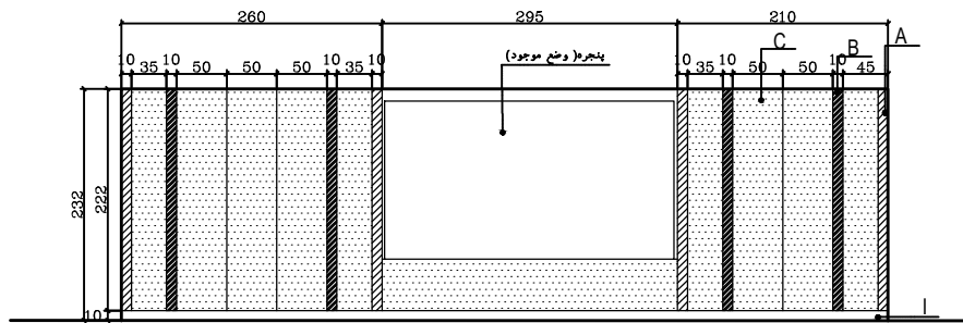
VIEW-A SCALE 1:20
