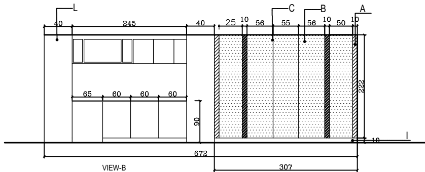
VIEW-B SCALE 1:20
